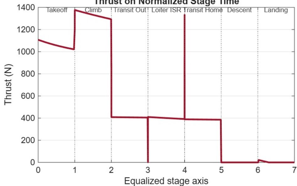
Thrust on Normalized Stage Time
