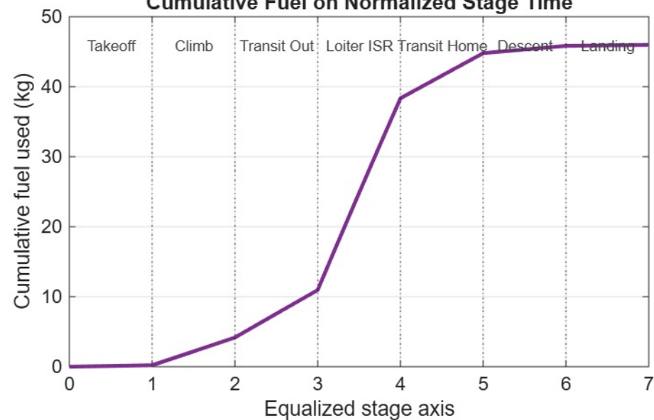
Cumulative Fuel on Normalized Stage Time
